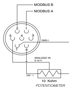
DETAIL CONNECTIONS
